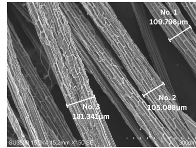
Figure 2. SEM image of secondary PALF ( liniwan ) at 150x magnification.
